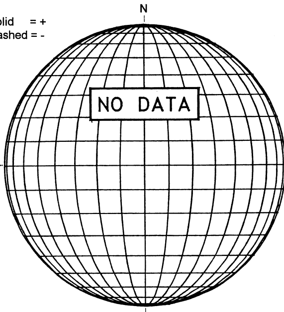
STANFORD MAGNETOGRAM
