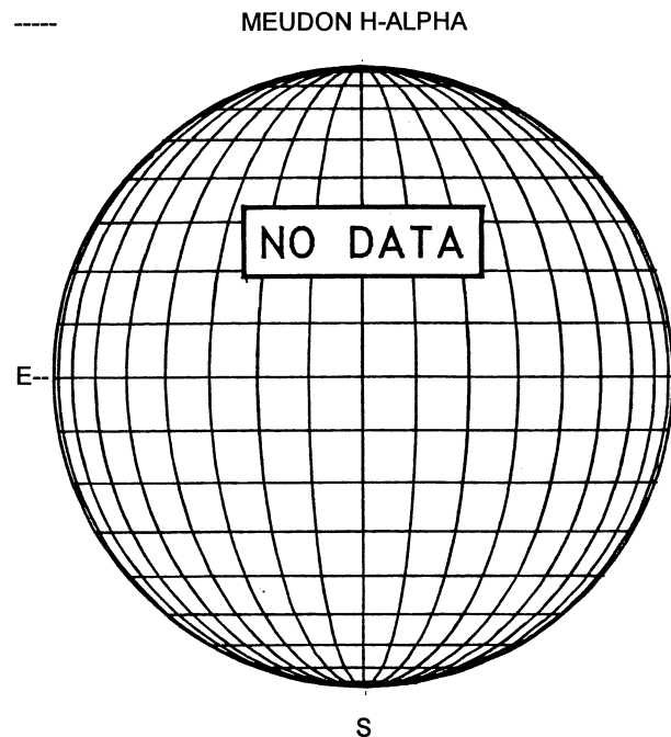
MEUDON H-ALPHA
